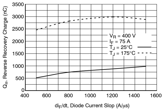
Figure 18. Stored Charge
