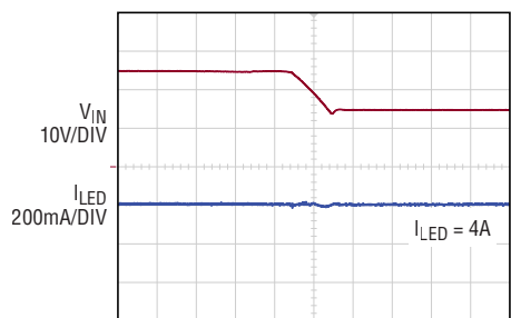
Input Voltage Transient Response
