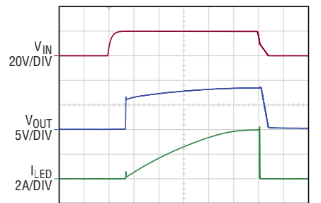
Turn-On and Turn-Off
