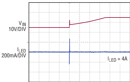
Input Voltage Transient Response
