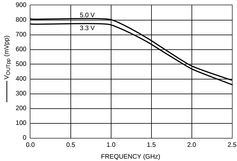
Figure 2. Typical V_{OUTTP} (mVpp) versus Frequency (GHz) @ 25°C
