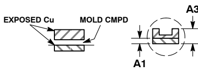
DETAIL B ALTERNATE CONSTRUCTIONS
