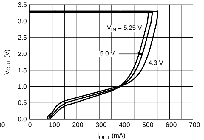
Figure 6. Output Voltage vs. Output Current 3.3 V Version ( T_J = 25^\circ\text{C} )
